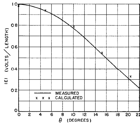
Fig. 8—Comparison of measured far-field pattern of horn and calculations based on near-field measurements with probe 4.
