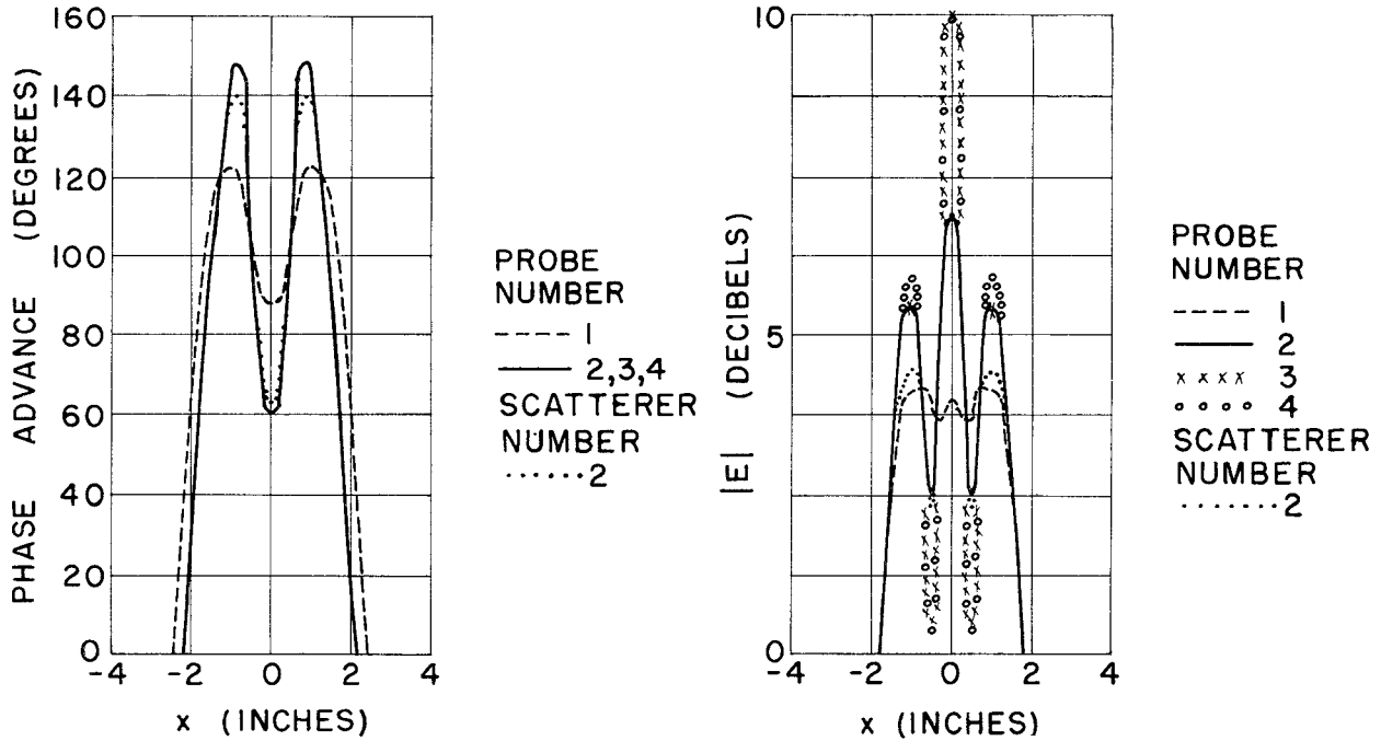
Fig. 5—Phase and amplitude distributions as measured with various probes and scatterer 2.
