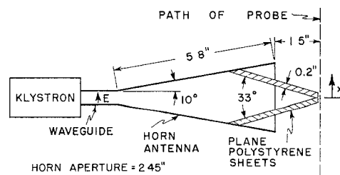
Fig. 1—Experimental arrangement for investigating probes.
