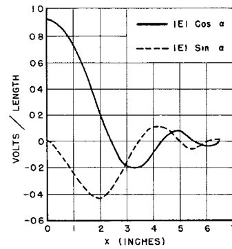
Fig. 7—Time-quadrature components of electric field of horn as measured with probe 4.
