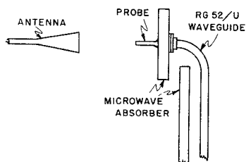
Fig. 2—Orientation of probe 4 and waveguide feed.
